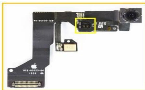
proximity sensor (mnf. unknown) 2.78 mm x 2.38 mm x 1.28 mm
