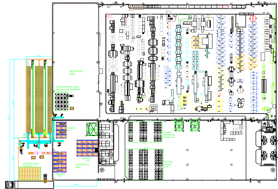
Site Ground View M 1:750
