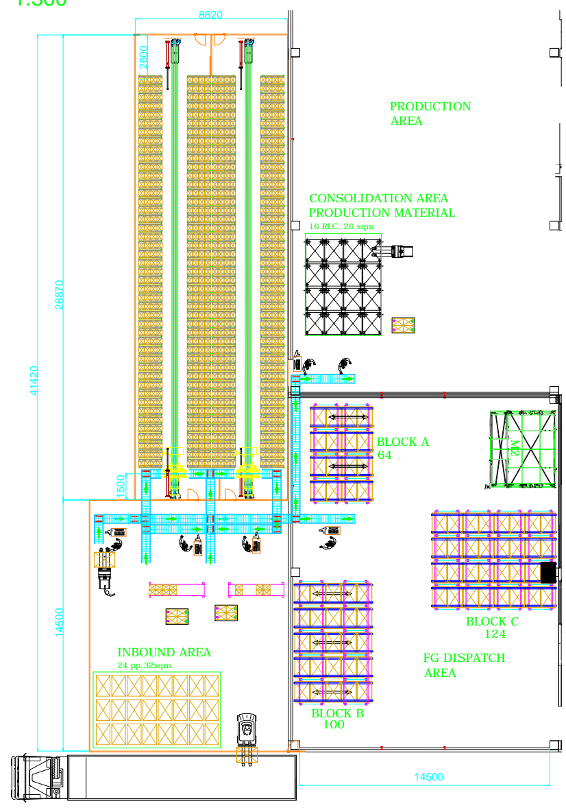
Warehouse Ground View 1:300
