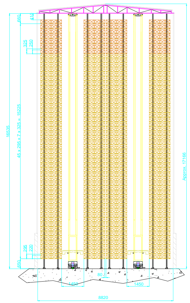
Cross Section M 1:150
