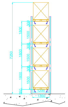
Section Finished goods M 1:150
