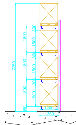
Section Finished goods M 1:150
