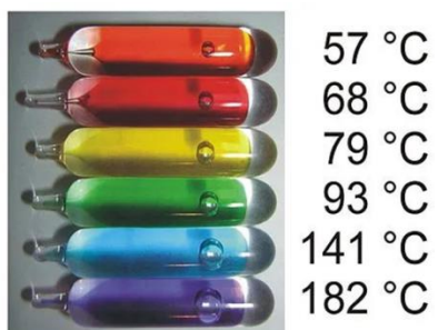
Slika 8. Prikaz staklene ampule, temperatura aktiviranja raspoznaje se po boji ampule https://blog.adafruit.com/2017/11/06/how-a-fire-sprinkler-works-including-color-coding-various-designs/ )
